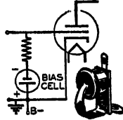
Bias cell and usage in typical circuit.
